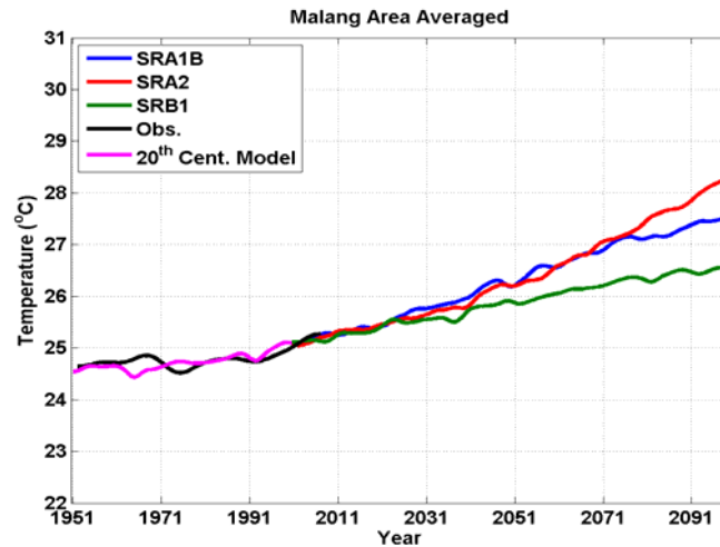
Figure 2. 13 The GCM out based projected temperature of Malang for the 21 st century with an extension back to 1951 (20 th century). Data has been smoothed to show only the long-term trend.
