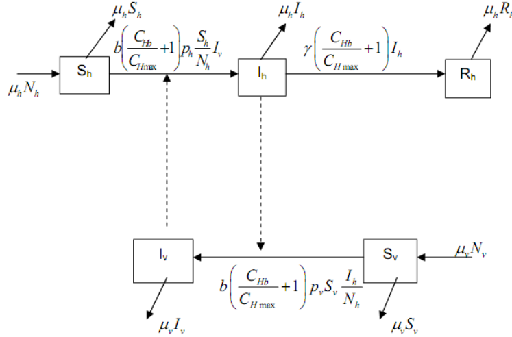
Figure 3. 2 Schematic of the compartment modeling of DHF
