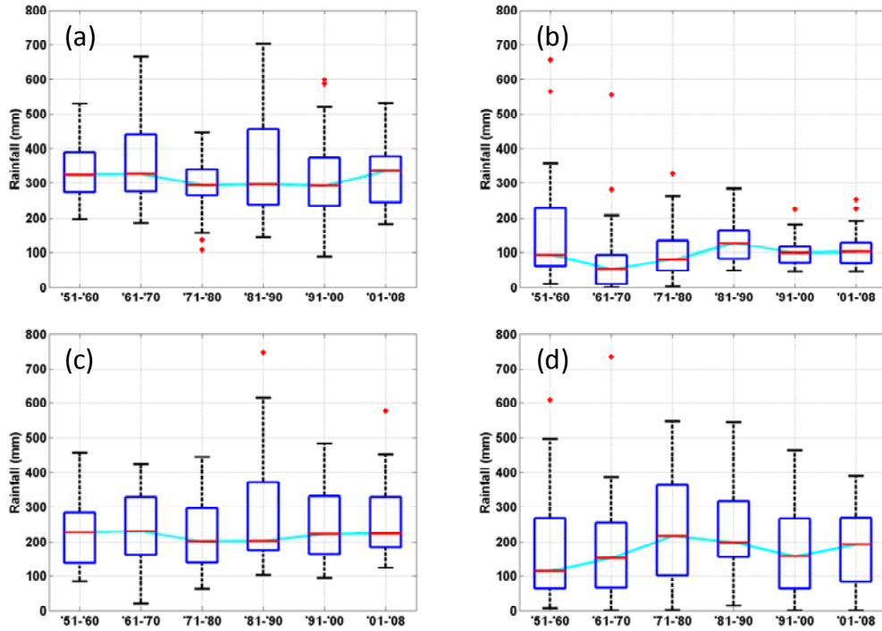
Figure 2. 5 Box-plot of inter-decadal rainfall time series of Malang (calculated from GPCC data) for (a) December-January-February, (b) June-July-August, (c) March-April-May, and (d) September-October-November. Each box represents the statistics of ten-year rainfall with cyan-colored lines connects the median values.
