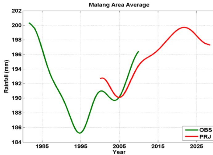
Figure 2.10 Similar to Figure 2.10 except for the results of CA method with smoothed time series of PUSAIR monthly rainfall (green) and SRES A1B analogue projection (red).
